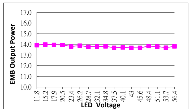
EMB Output Power V.S. LED Voltage
