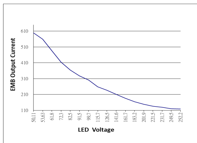
EMB Output Current V.S. LED Voltage
