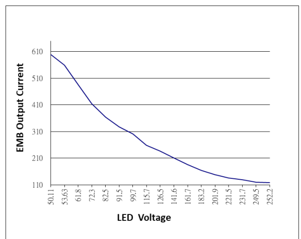
EMB Output Current V.S. LED Voltage
