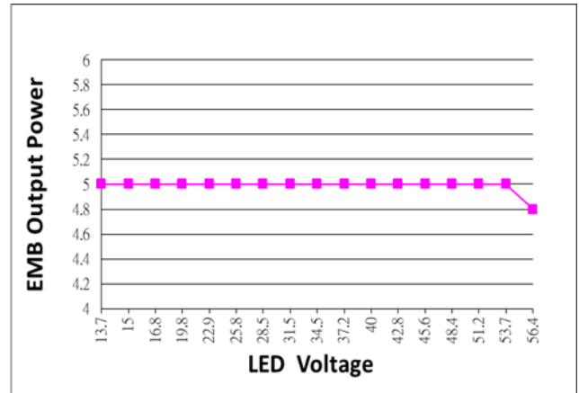
EMB Output Power V.S. LED Voltage
