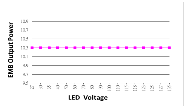
Power Output Power V.S. LED Voltage
