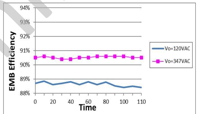
EMB Efficiency V.S. Time
