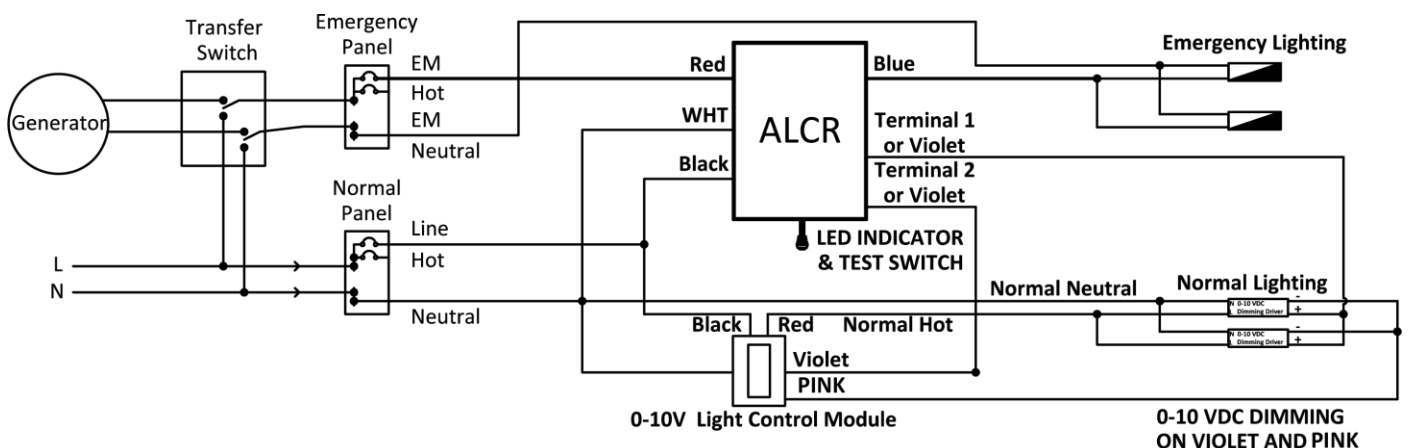
(A) With 0-10V Dimmer
