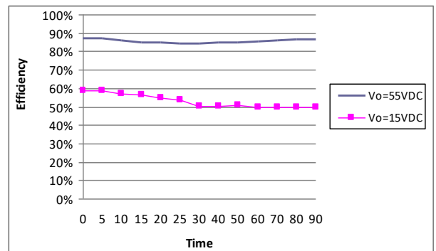
LED Efficiency V.S. Time
