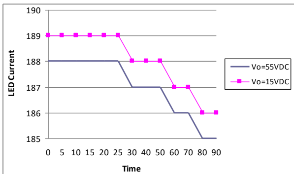
LED Current V.S. Time
