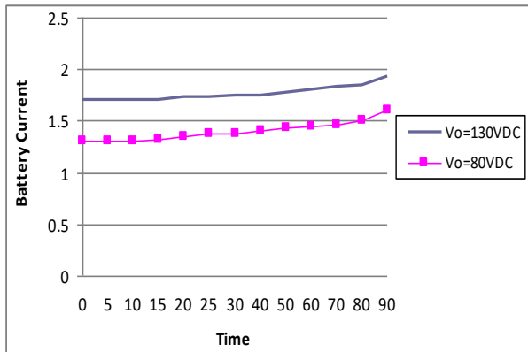
Battery Current V.S. Time
