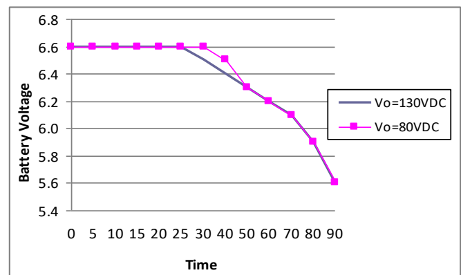
Battery Voltage V.S. Time
