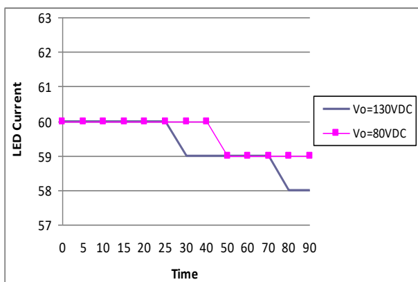
LED Current V.S. Time
