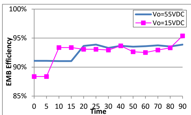
EMB Efficiency V.S. Time
