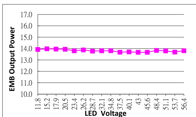
EMB Output Power V.S. LED Voltage
