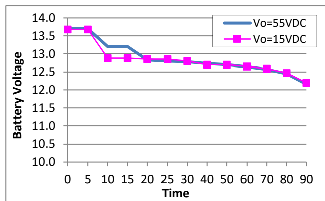
Battery Voltage V.S. Time
