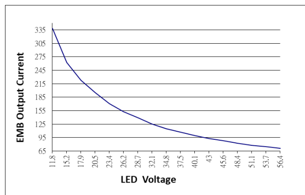
EMB Output Current V.S. LED Voltage
