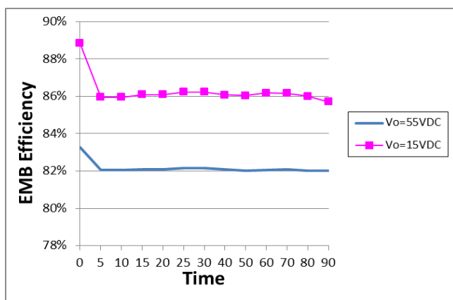
EMB Efficiency V.S. Time
