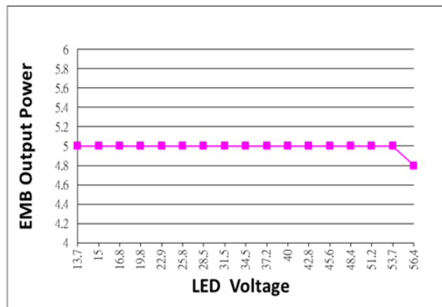
EMB Output Power V.S. LED Voltage
