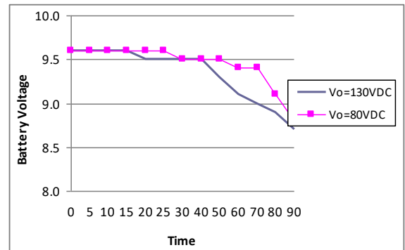
Battery Voltage V.S. Time
