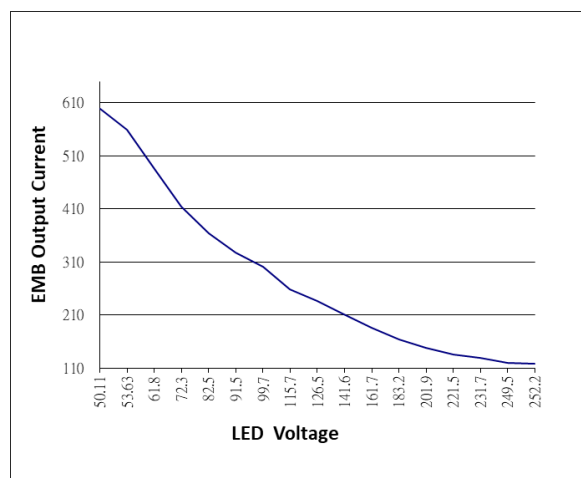
EMB Output Current V.S. LED Voltage
