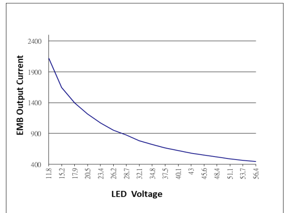
EMB Output Current V.S. LED Voltage
