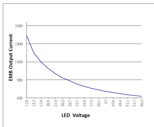
EMB Output Current V.S. LED Voltage
