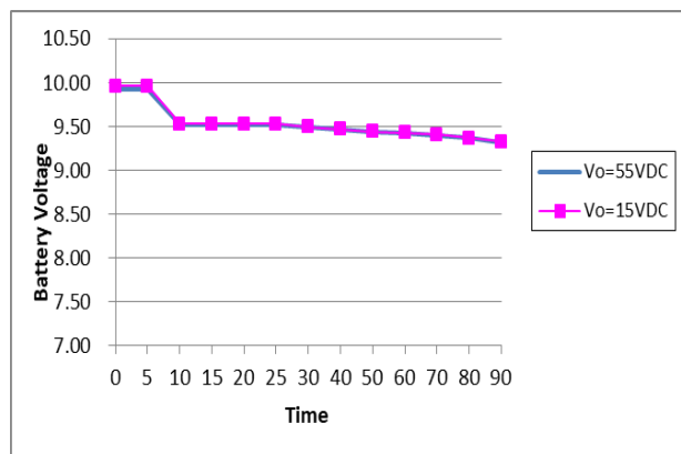
Battery Voltage V.S. Time
