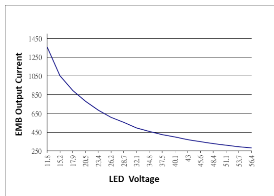
EMB Output Current V.S. LED Voltage
