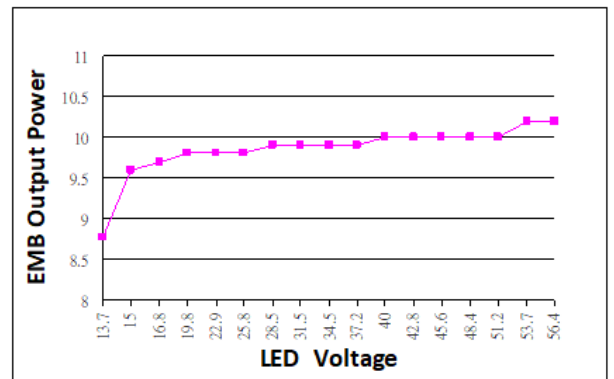
EMB Output Power V.S. LED Voltage
