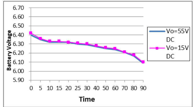
Battery Voltage V.S. Time
