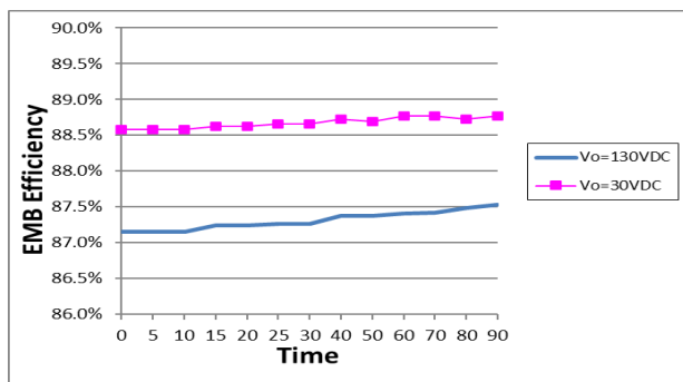
EMB Efficiency V.S. Time
