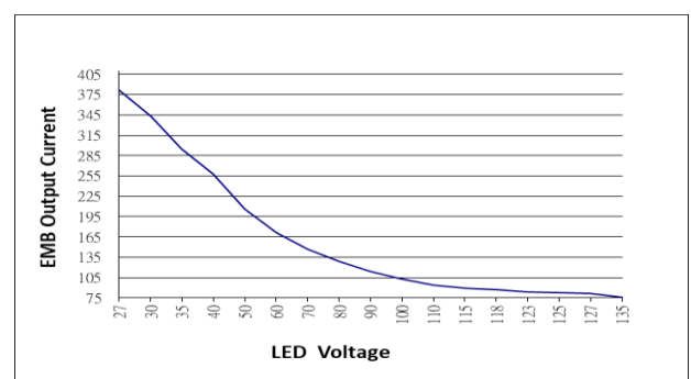
EMB Output Current V.S. LED Voltage
